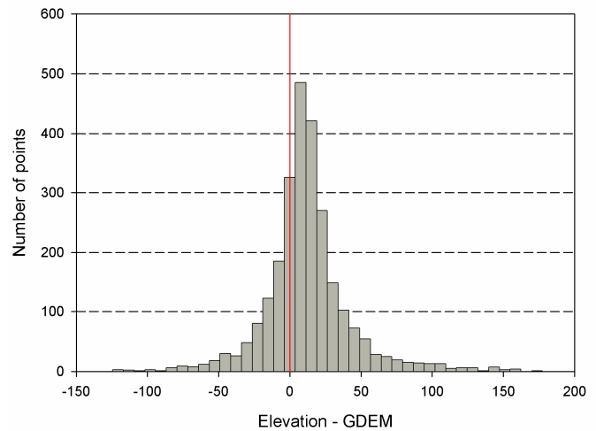
Figure 2. Histogram of control points heights minus GDEM heights. Some statistics for this distribution: D of Kolmogorov-Smirnov test=0.1165; p < 0.01 , Lilliefors- p < 0.01 ; number of elements=2592; Mean=12.33; Standard deviation=30.62; Maximum=177.47; Minimum=-124.45 and Shapiro-Wilk test W=0.91 ; p=0.00 .
