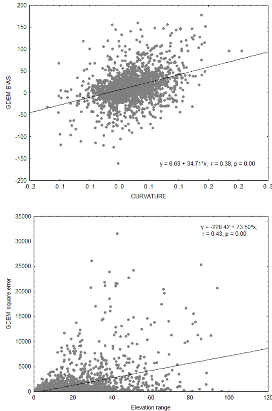
Figure 3. Relationship between GDEM bias-curvature (upper plot) and GDEM square error-elevation range (lower plot). Curvature was calculated with Zevenbergen and Thorne method [9] while elevation range was calculated as the difference between the highest and lowest elevations in a window of 5x5 cells. Both of them, curvature and elevation range, were calculated from the MTN DEM and then related to control points estimated bias and square error.
